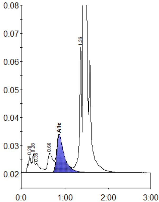
Peak table - ID: 10347399
